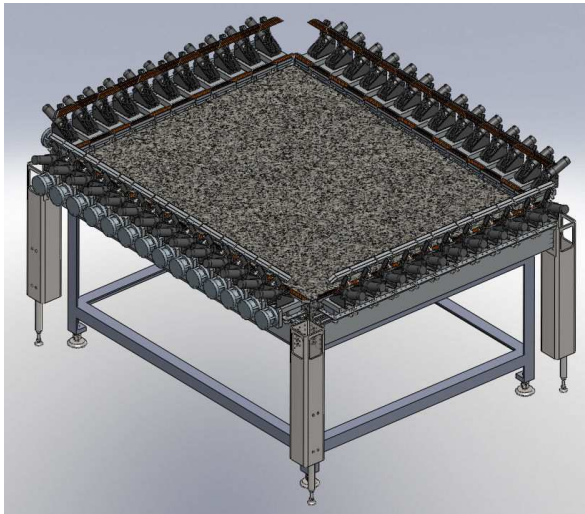
Model SS-50 Screen Stretcher
